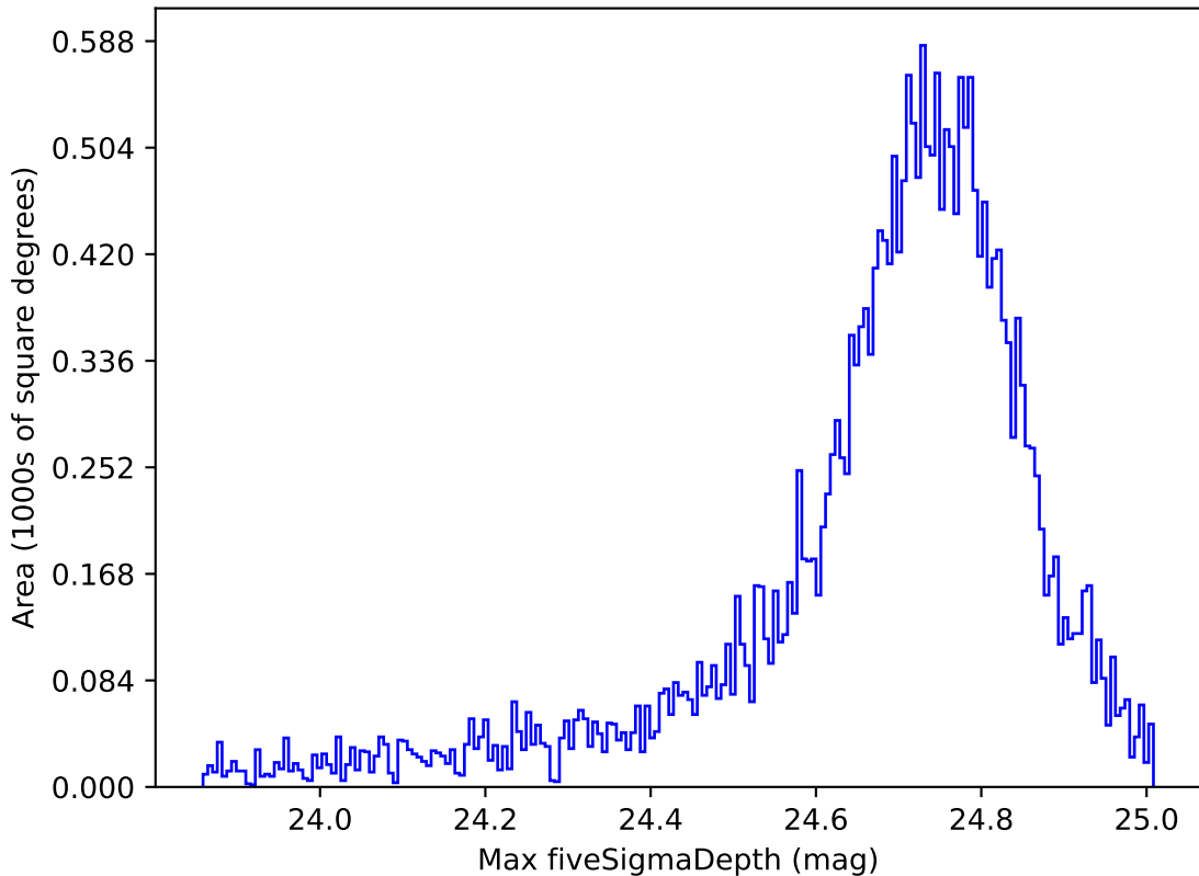
ddf_acor_sf20_lsf30_lsr50_v3.4_10yrs All sky r band: Max fiveSigmaDepth
