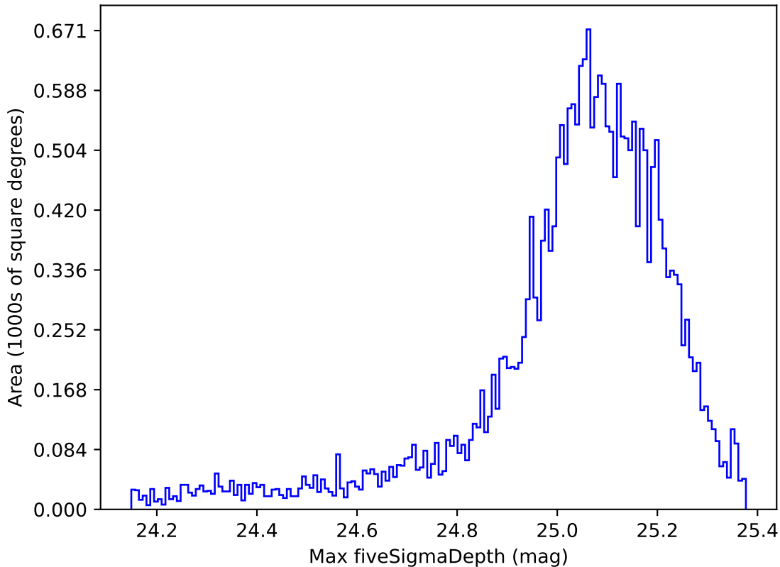
ddf_acor_sf20_lsf30_lsr50_v3.4_10yrs All sky g band: Max fiveSigmaDepth
