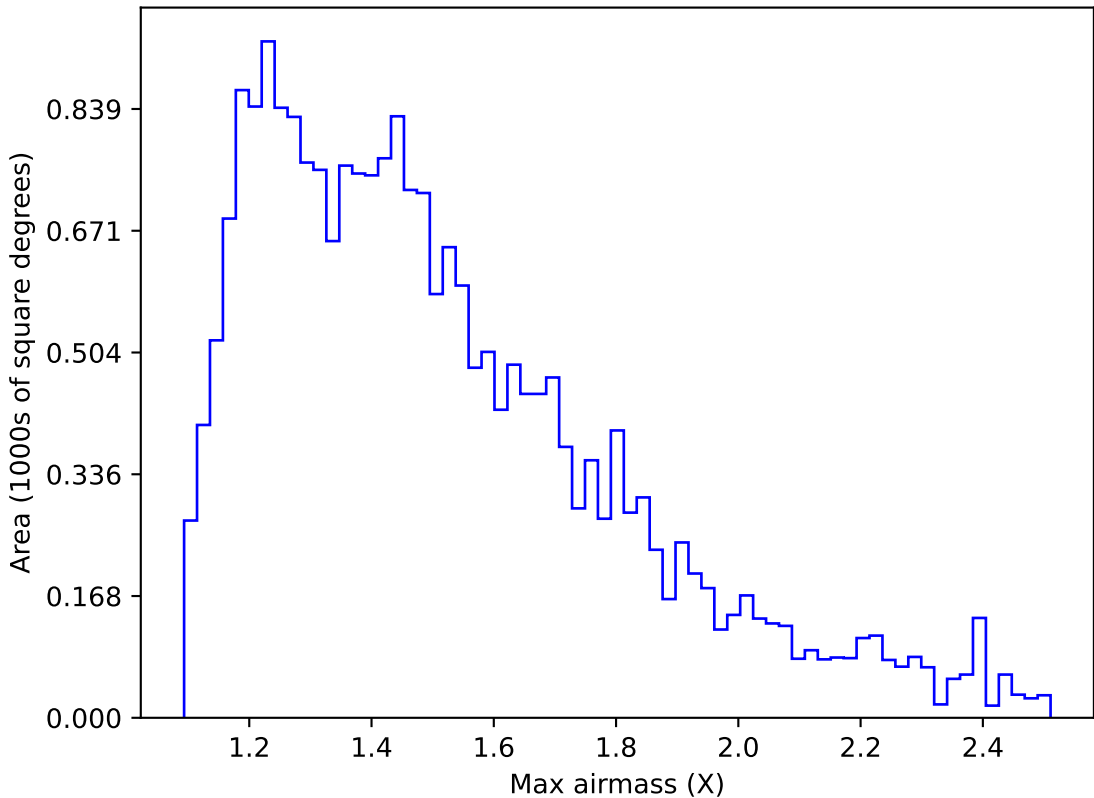
ddf_acor_sf20_lsf30_lsr50_v3.4_10yrs Yr 1 u band: Max airmass
