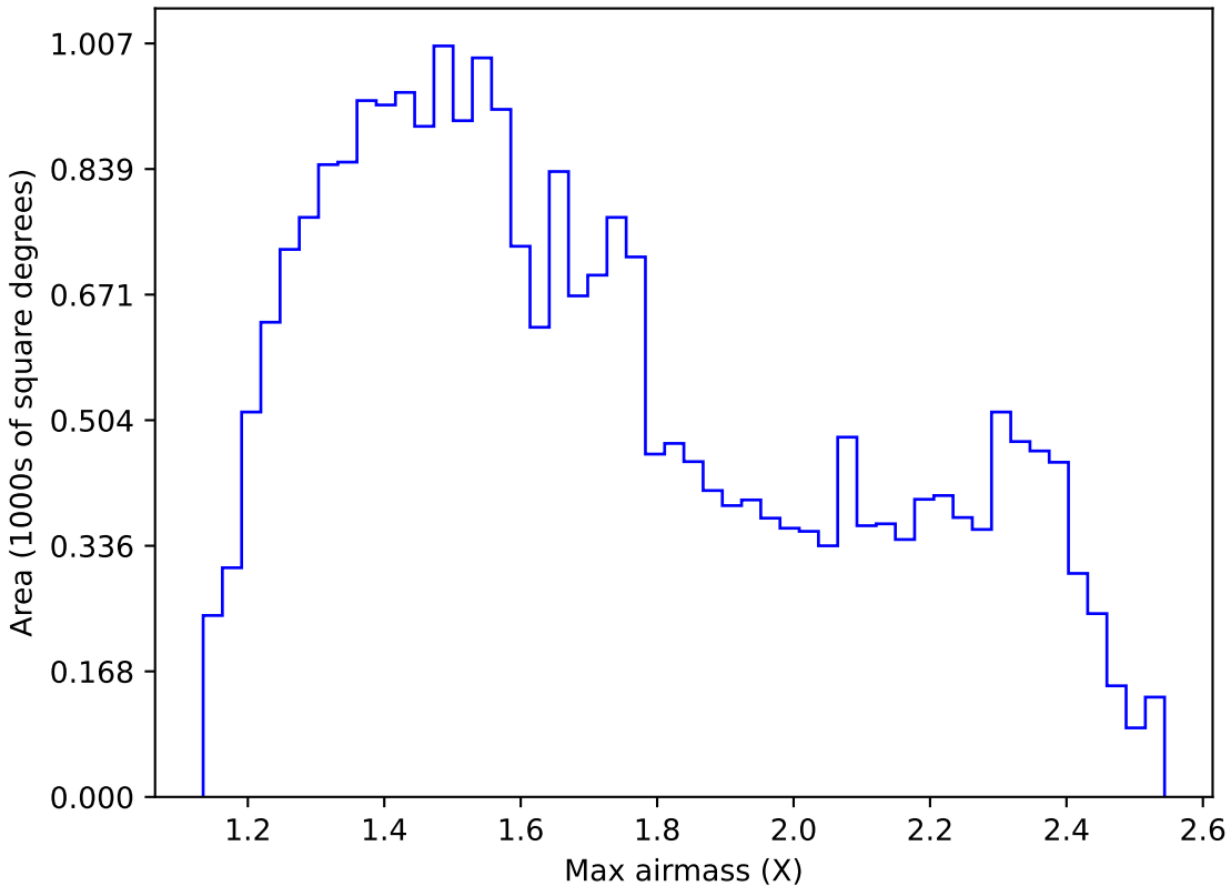
ddf_acor_sf20_lsf30_lsr50_v3.4_10yrs Yr 1 r band: Max airmass
