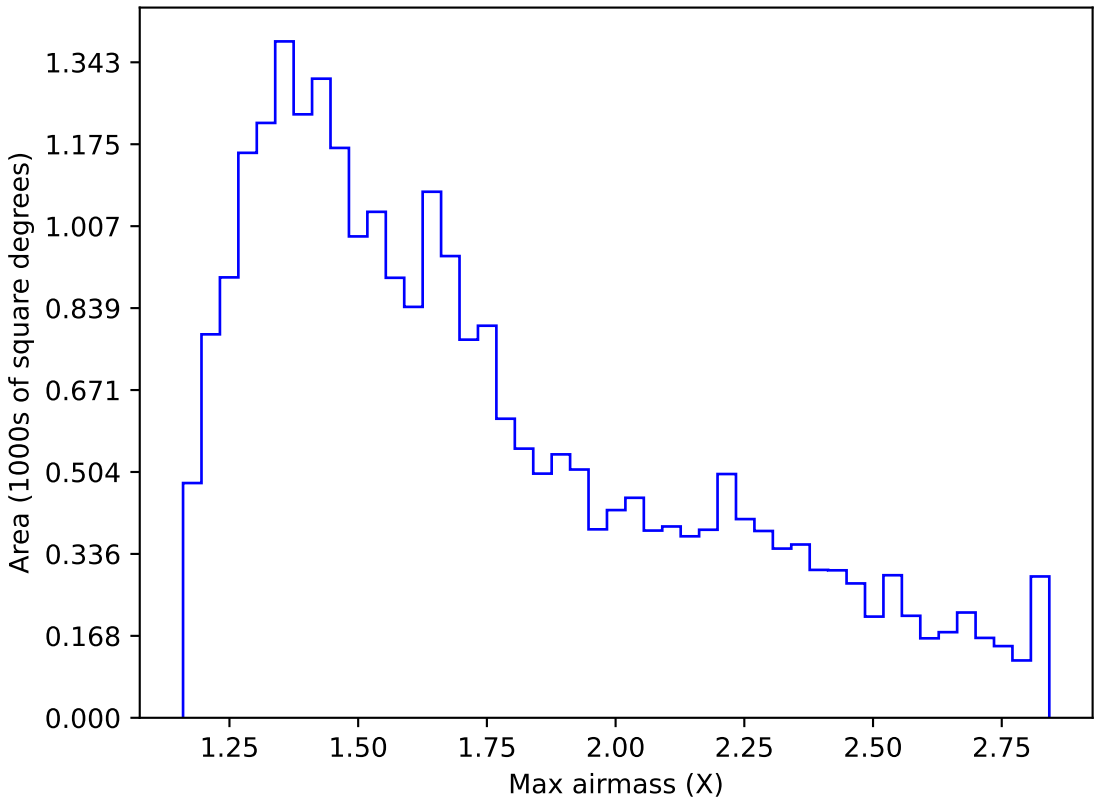
ddf_acor_sf20_lsf30_lsr50_v3.4_10yrs Yr 1 i band: Max airmass
