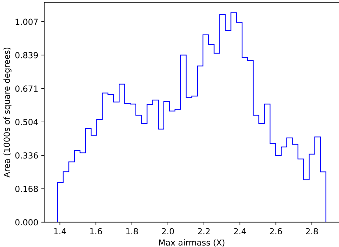
ddf_acor_sf20_lsf30_lsr50_v3.4_10yrs Yr 1 all bands: Max airmass
