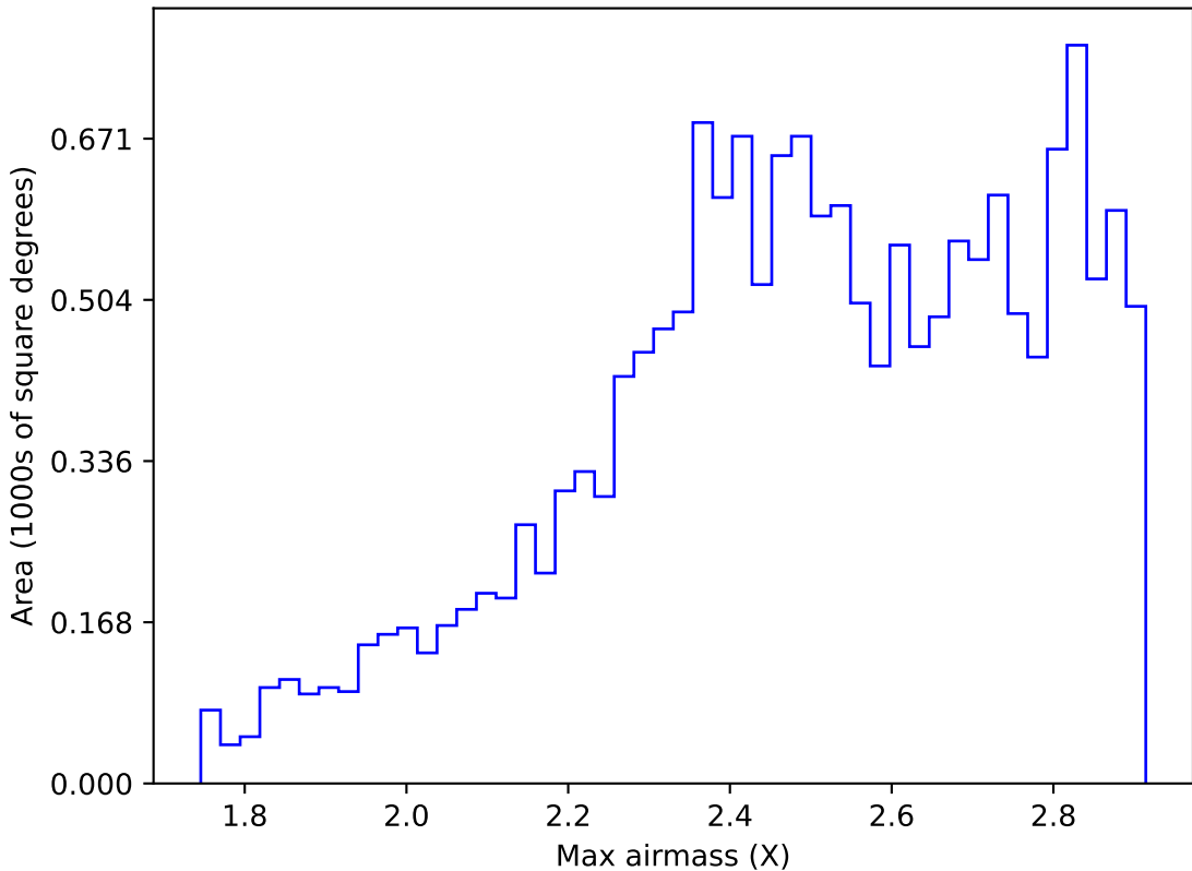
ddf_acor_sf20_lsf30_lsr50_v3.4_10yrs WFD z band: Max airmass
