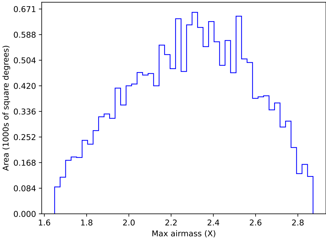
ddf_acor_sf20_lsf30_lsr50_v3.4_10yrs WFD y band: Max airmass
