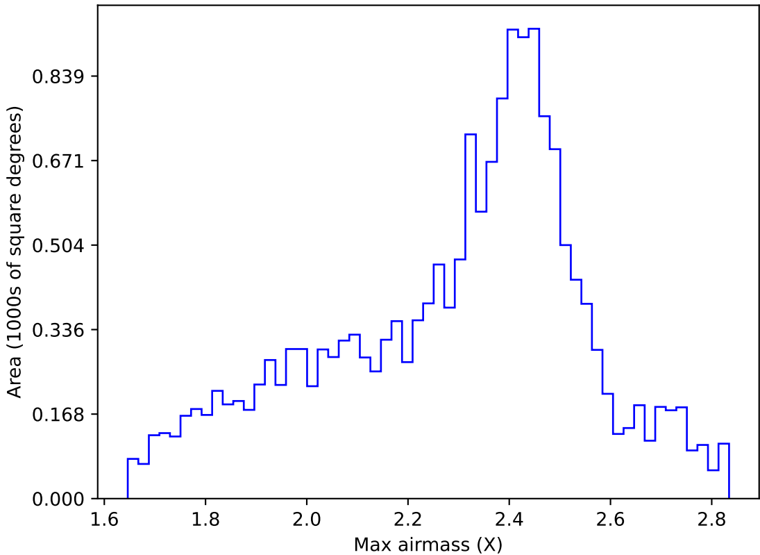
ddf_acor_sf20_lsf30_lsr50_v3.4_10yrs WFD r band: Max airmass
