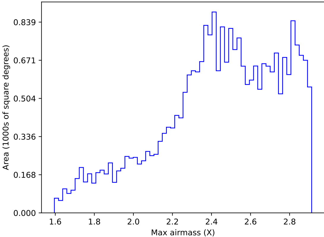
ddf_acor_sf20_lsf30_lsr50_v3.4_10yrs All sky z band: Max airmass
