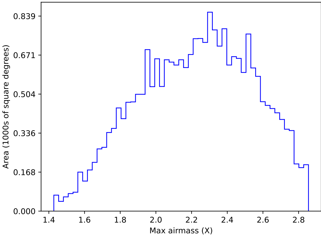
ddf_acor_sf20_lsf30_lsr50_v3.4_10yrs All sky y band: Max airmass
