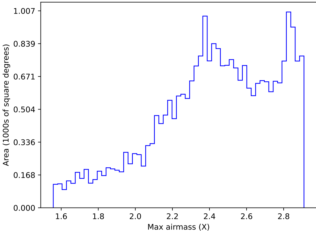
ddf_acor_sf20_lsf30_lsr50_v3.4_10yrs All sky i band: Max airmass
