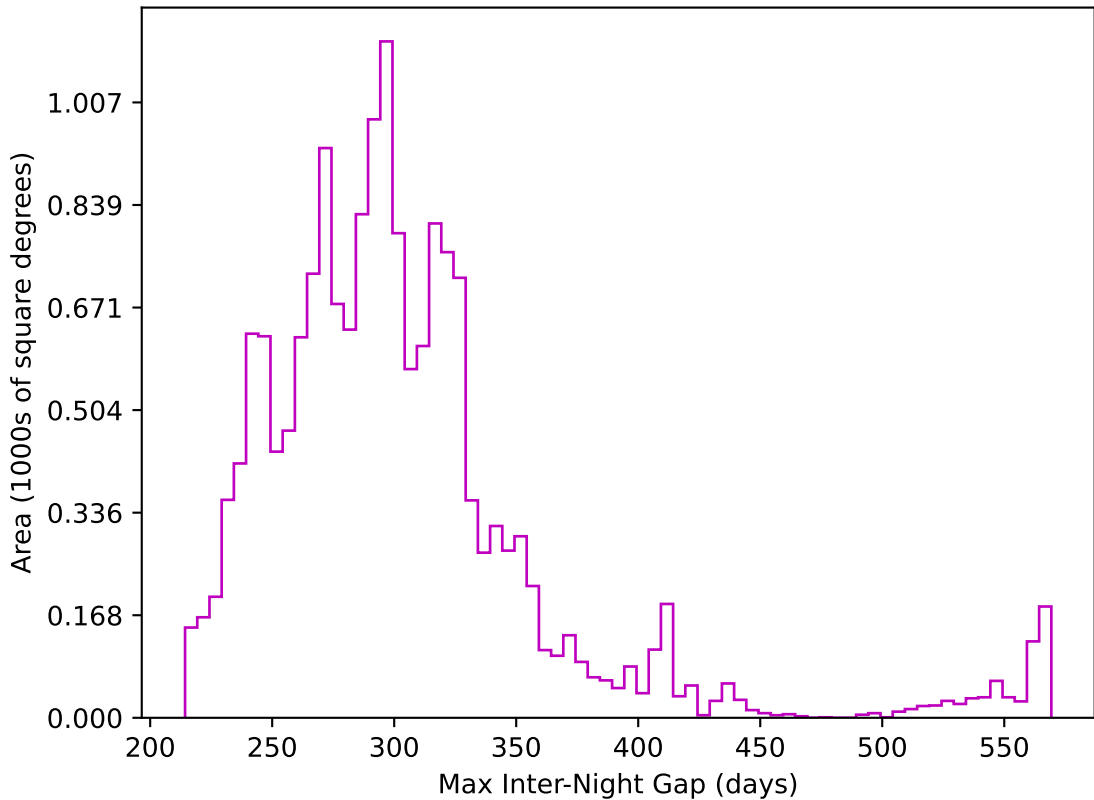
ddf_acor_sf20_lsf30_lsr50_v3.4_10yrs WFD z band: Max Inter-Night Gap
