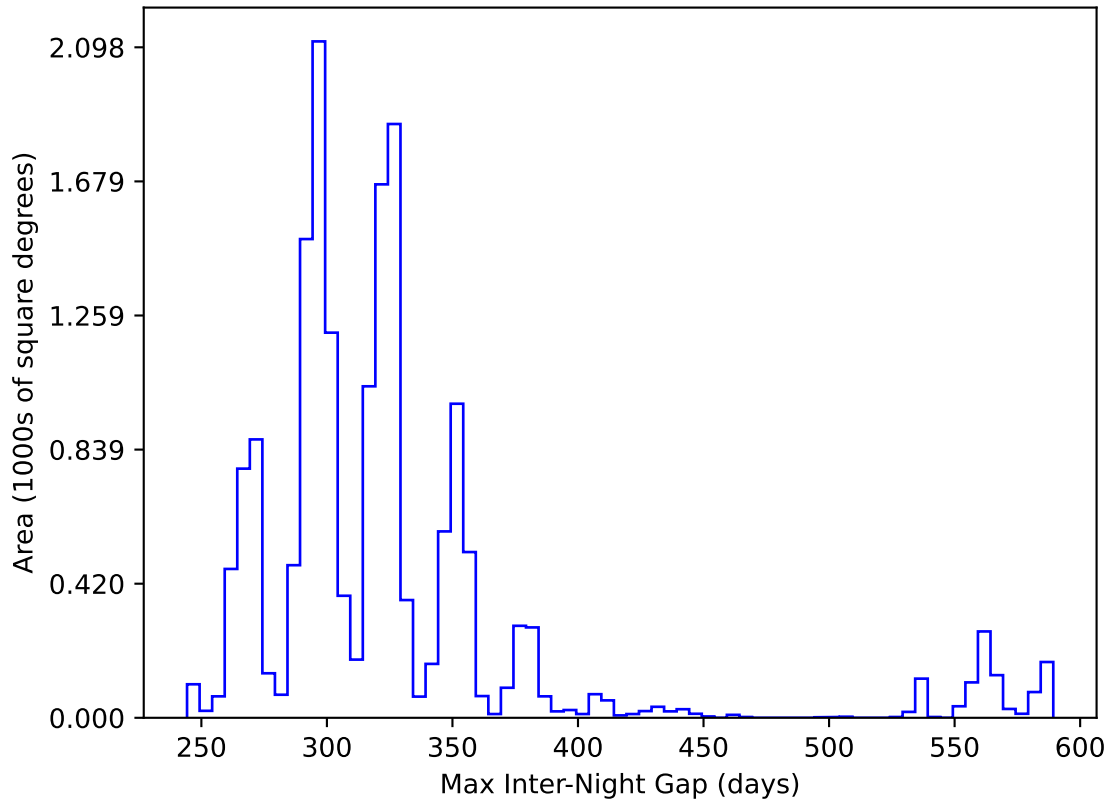
ddf_acor_sf20_lsf30_lsr50_v3.4_10yrs WFD y band: Max Inter-Night Gap
