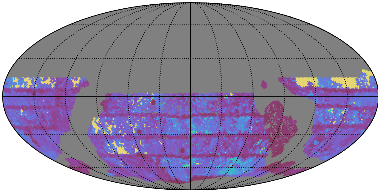
ddf_acor_sf20_lsf30_lsr50_v3.4_10yrs WFD r band: Max Inter-Night Gap
