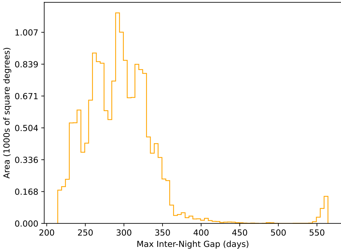
ddf_acor_sf20_lsf30_lsr50_v3.4_10yrs WFD r band: Max Inter-Night Gap
