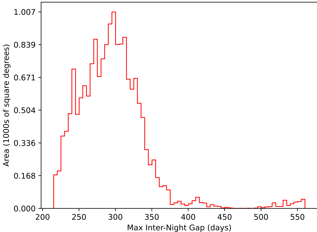
ddf_acor_sf20_lsf30_lsr50_v3.4_10yrs WFD i band: Max Inter-Night Gap
