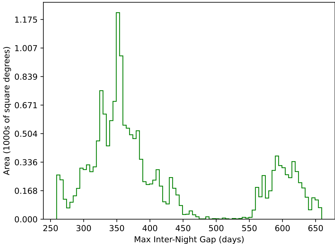
ddf_acor_sf20_lsf30_lsr50_v3.4_10yrs WFD g band: Max Inter-Night Gap
