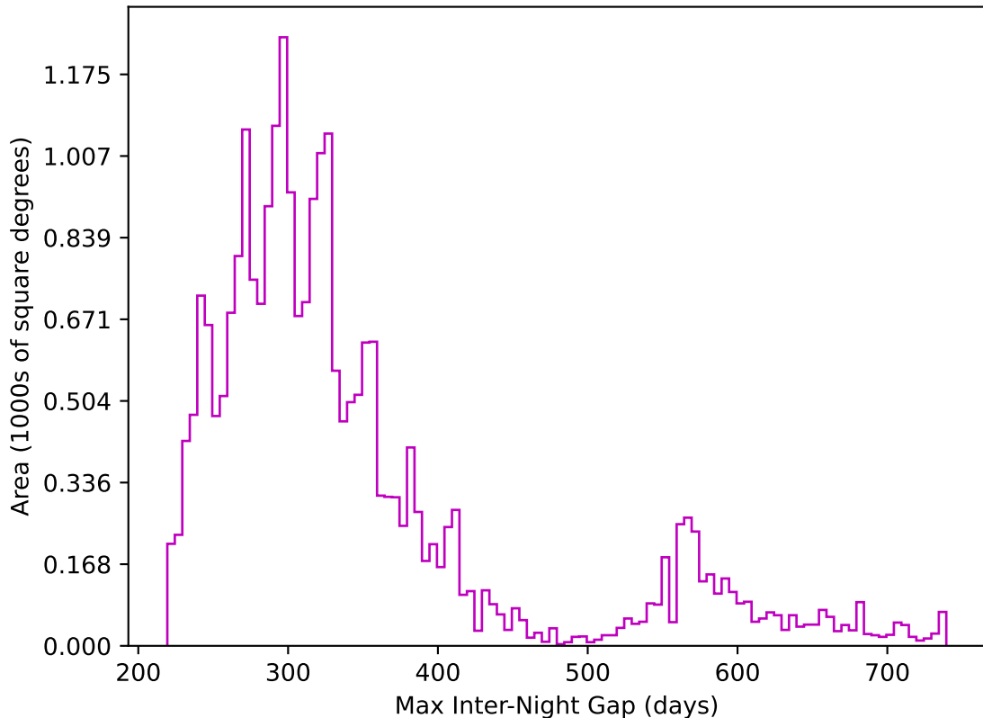
ddf_acor_sf20_lsf30_lsr50_v3.4_10yrs All sky z band: Max Inter-Night Gap
