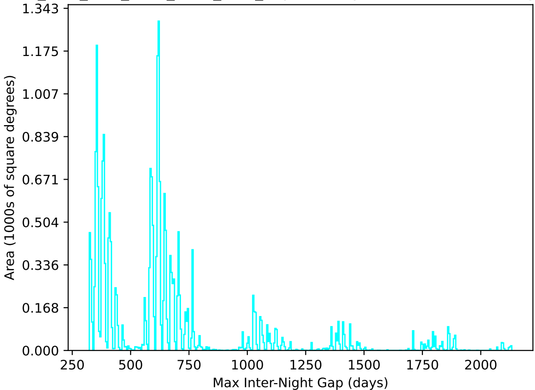
ddf_acor_sf20_lsf30_lsr50_v3.4_10yrs All sky u band: Max Inter-Night Gap
