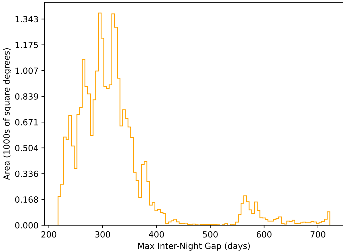
ddf_acor_sf20_lsf30_lsr50_v3.4_10yrs All sky r band: Max Inter-Night Gap
