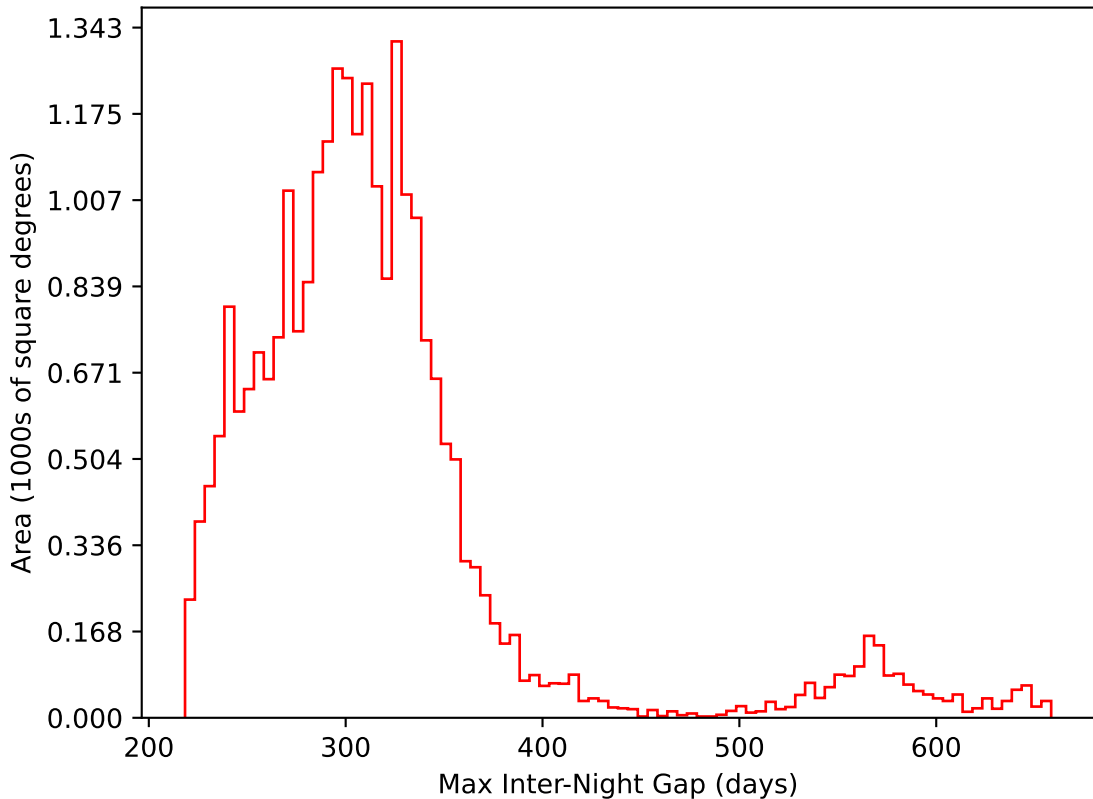
ddf_acor_sf20_lsf30_lsr50_v3.4_10yrs All sky i band: Max Inter-Night Gap
