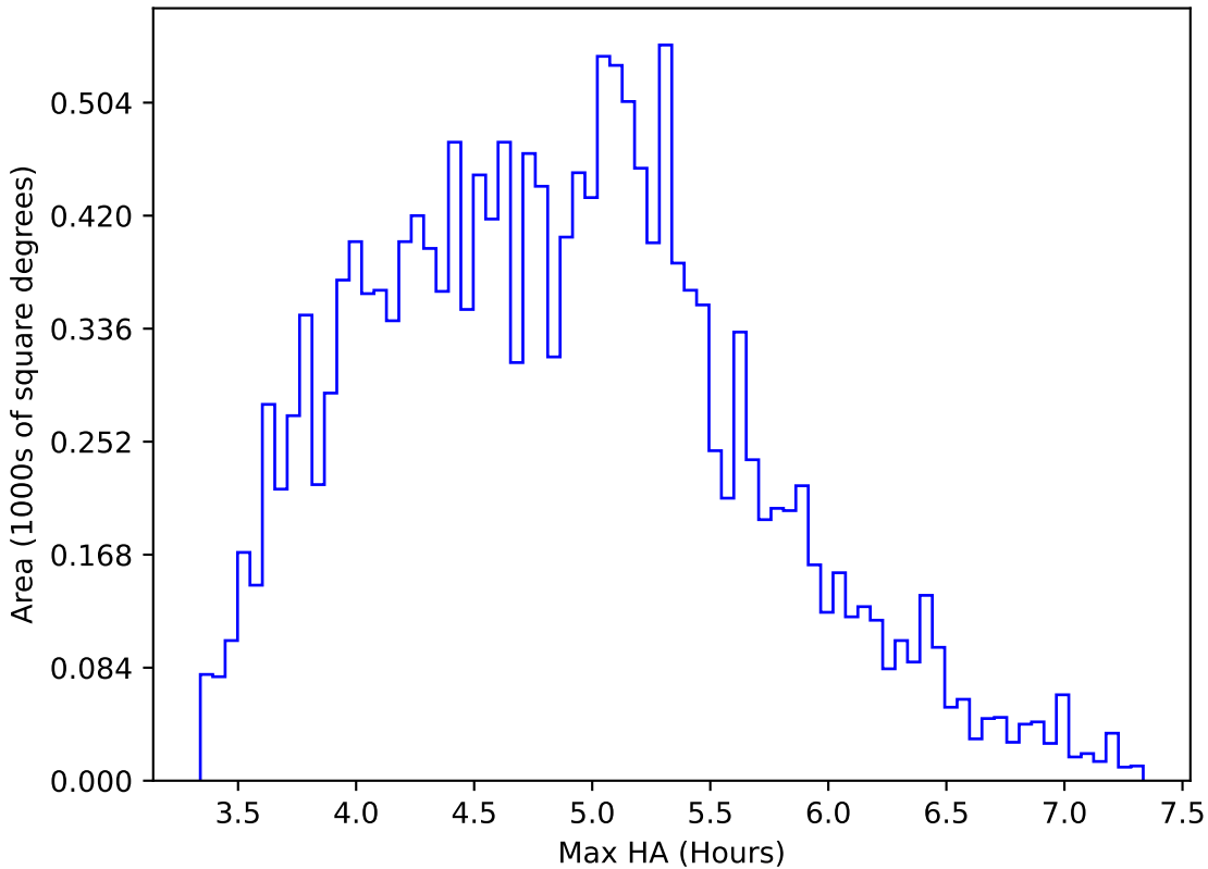
ddf_acor_sf20_lsf30_lsr50_v3.4_10yrs WFD z band: Max HA
