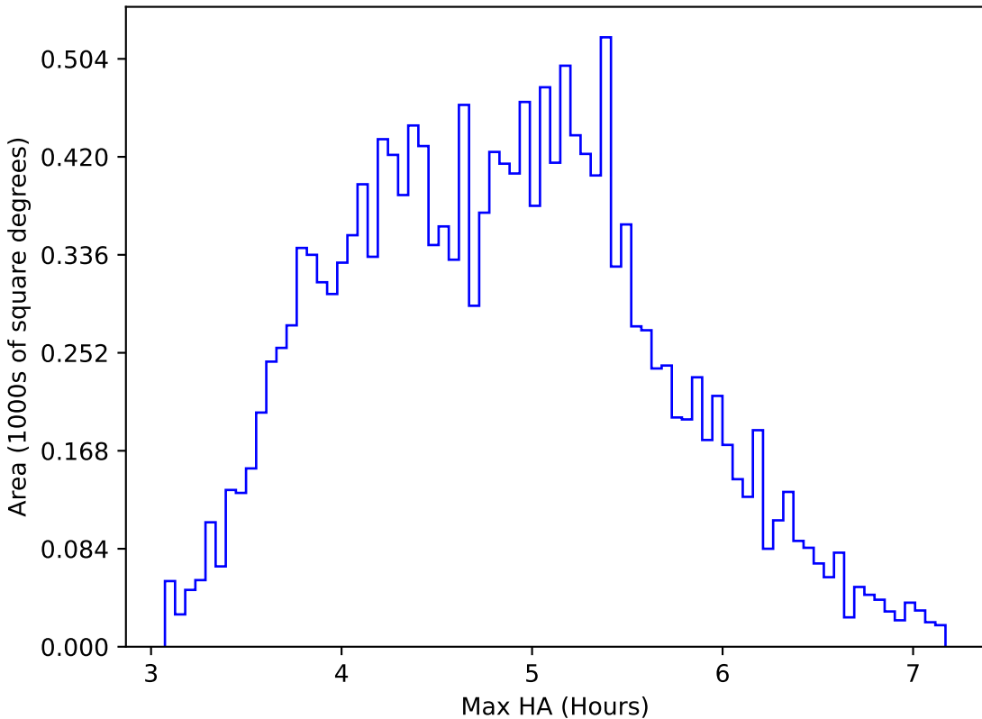
ddf_acor_sf20_lsf30_lsr50_v3.4_10yrs WFD i band: Max HA
