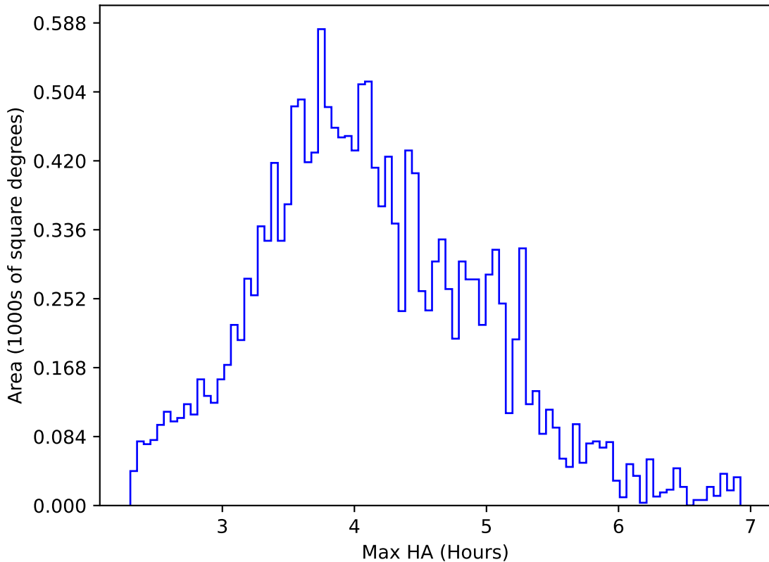
ddf_acor_sf20_lsf30_lsr50_v3.4_10yrs WFD g band: Max HA
