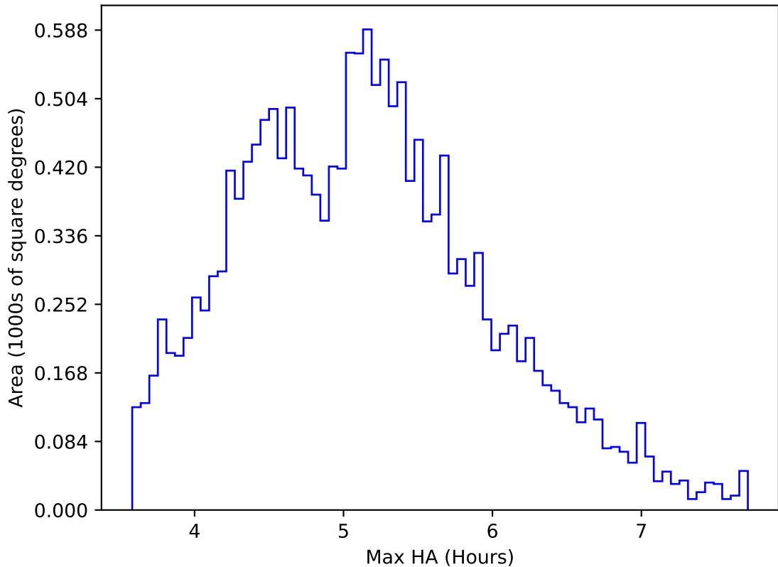
ddf_acor_sf20_lsf30_lsr50_v3.4_10yrs WFD all bands: Max HA
