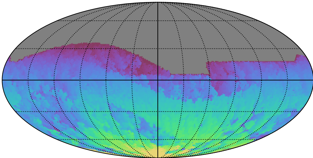
ddf_acor_sf20_lsf30_lsr50_v3.4_10yrs All sky z band: Max HA
