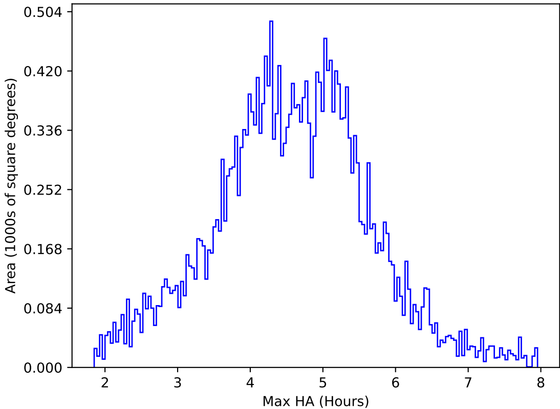
ddf_acor_sf20_ls30_lsr50_v3.4_10yrs All sky z band: Max HA
