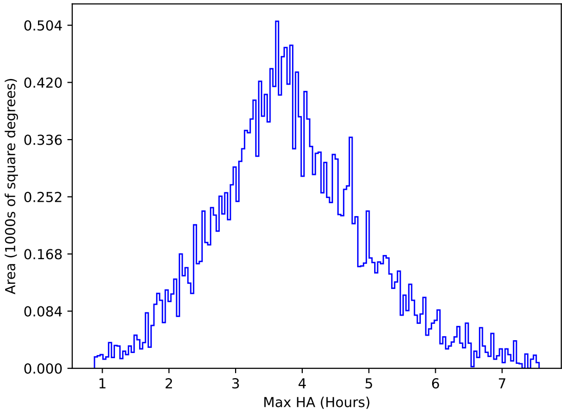
ddf_acor_sf20_lsf30_lsr50_v3.4_10yrs All sky u band: Max HA
