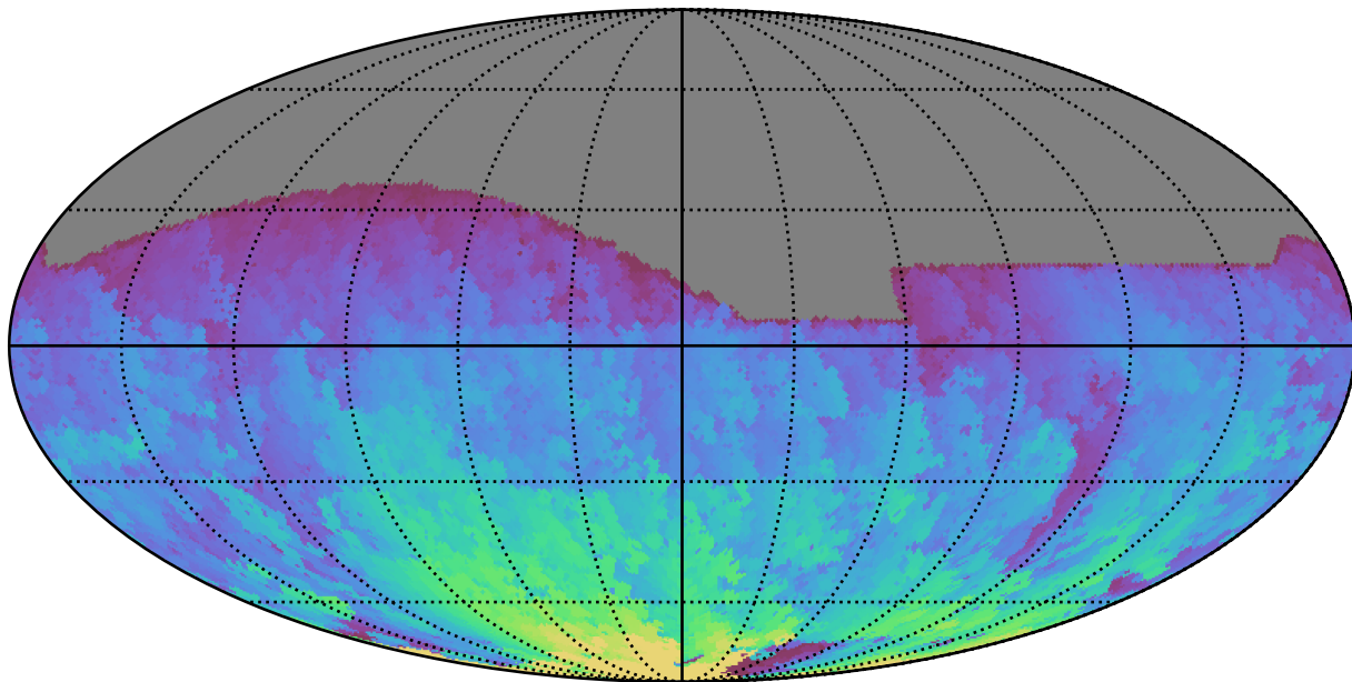
ddf_acor_sf20_lsf30_lsr50_v3.4_10yrs All sky r band: Max HA
