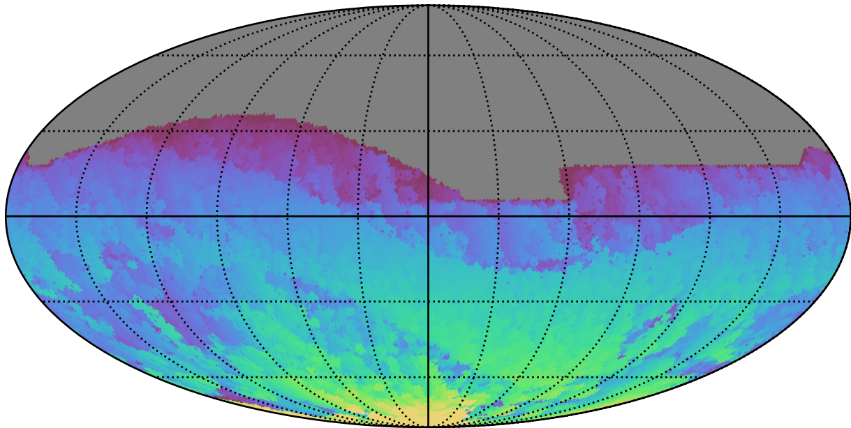
ddf_acor_sf20_lsf30_lsr50_v3.4_10yrs All sky i band: Max HA
