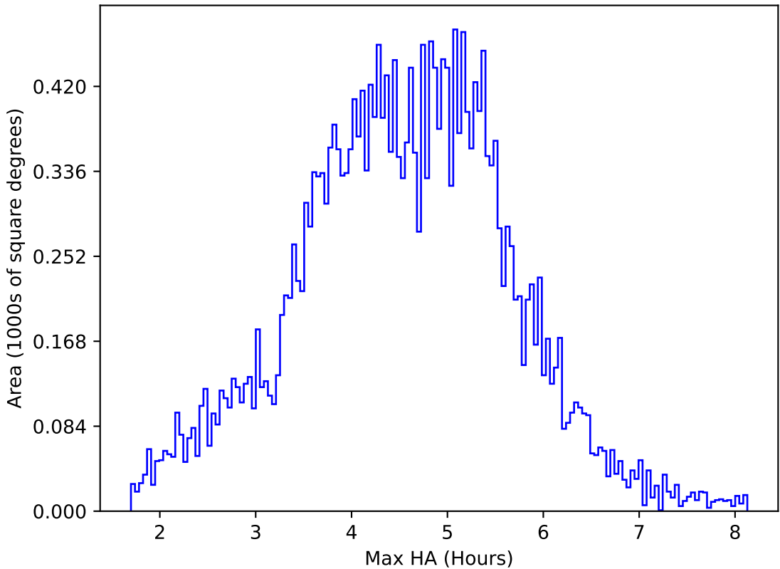
ddf_acor_sf20_lsf30_lsr50_v3.4_10yrs All sky i band: Max HA
