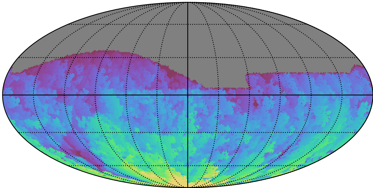
ddf_acor_sf20_lsf30_lsr50_v3.4_10yrs All sky g band: Max HA
