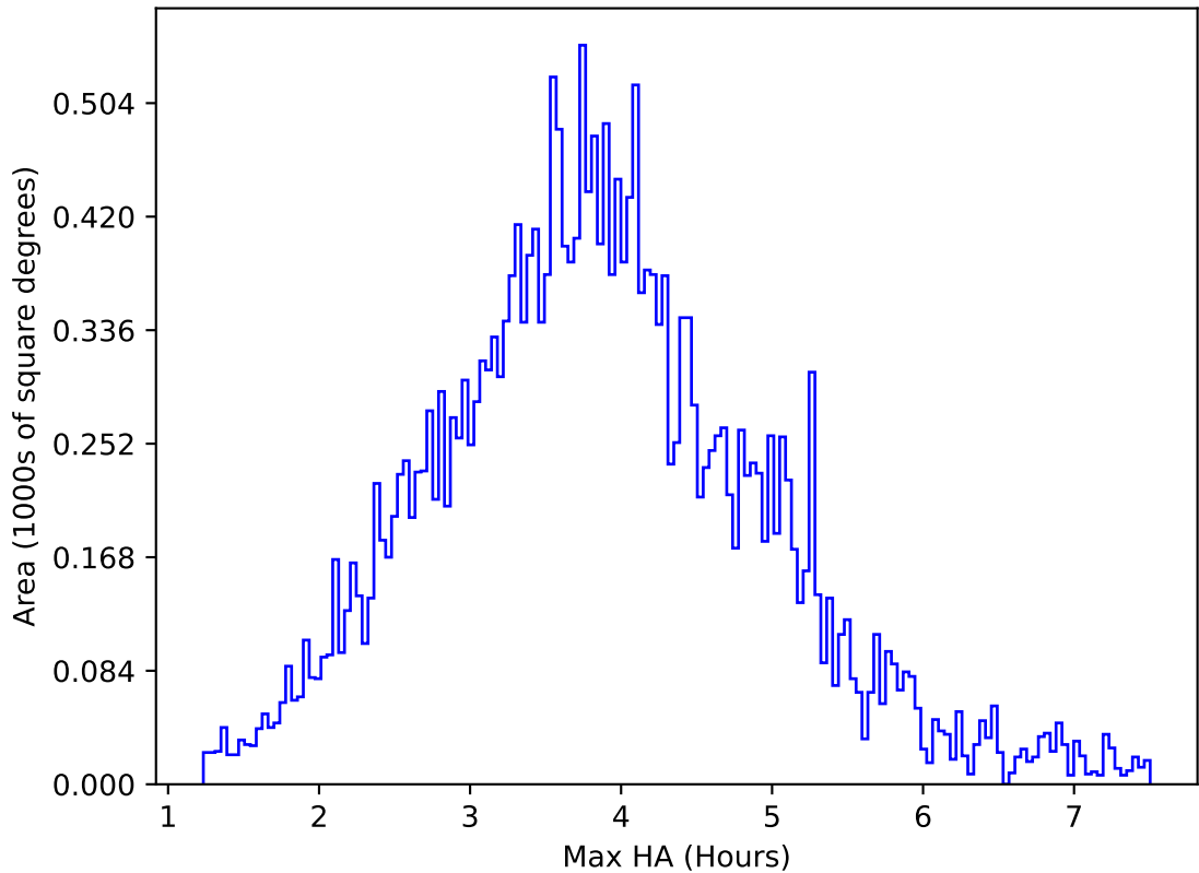
ddf_acor_sf20_lsf30_lsr50_v3.4_10yrs All sky g band: Max HA
