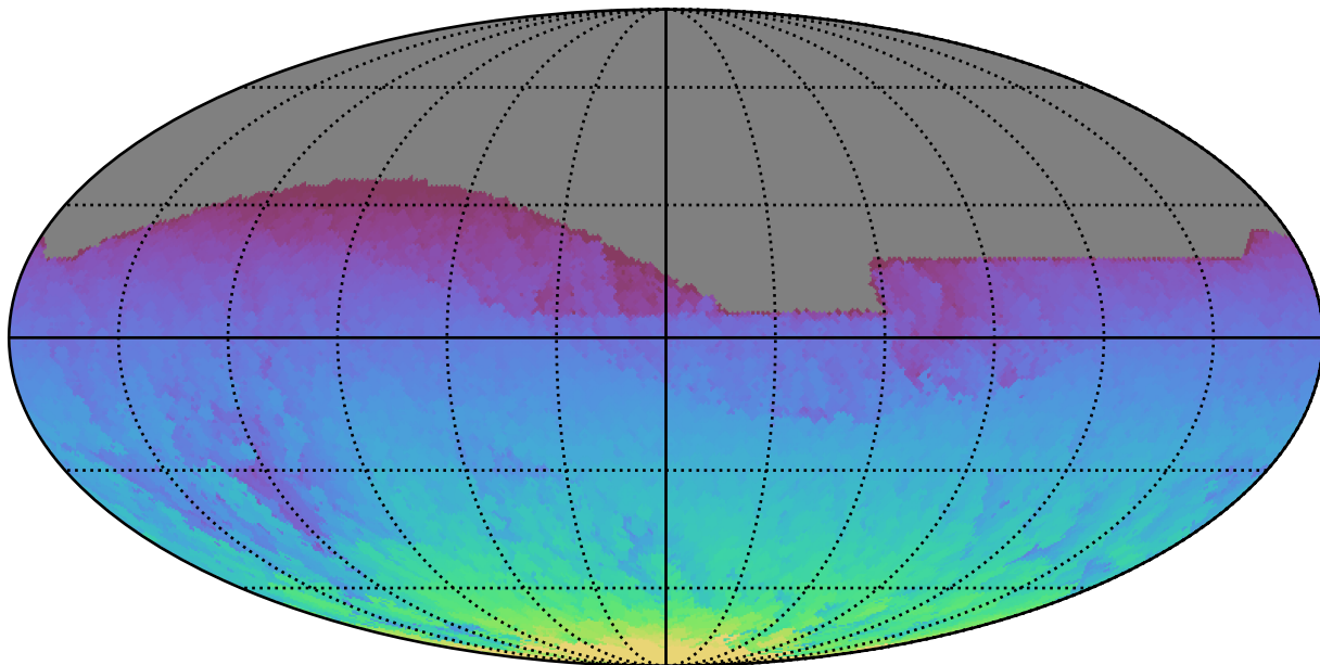
ddf_acor_sf20_lsf30_lsr50_v3.4_10yrs All sky all bands: Max HA
