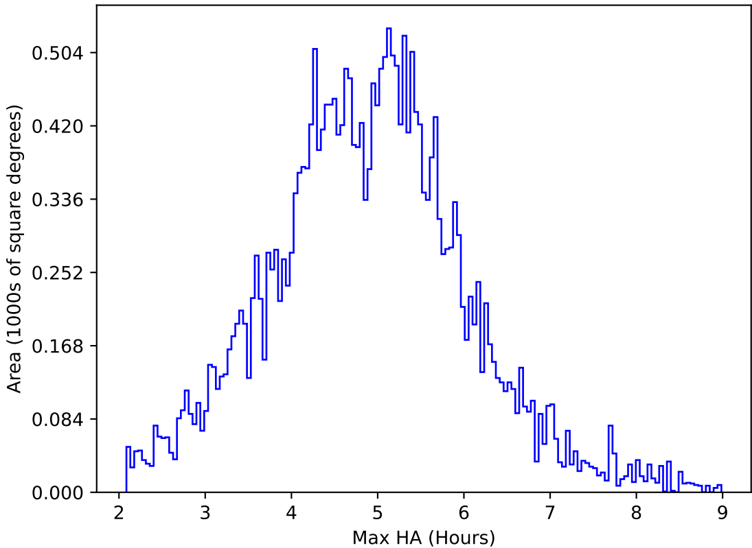
ddf_acor_sf20_lsf30_lsr50_v3.4_10yrs All sky all bands: Max HA
