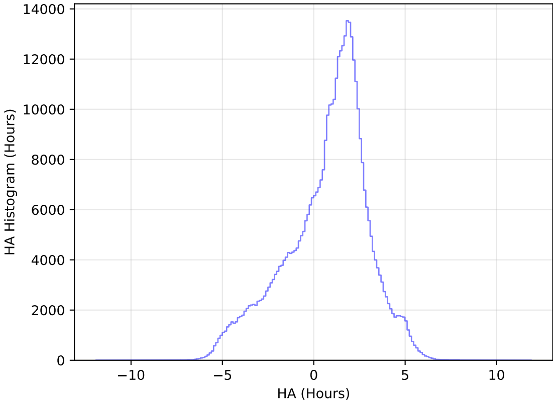
ddf_acor_sf20_lsf30_lsr50_v3.4_10yrs WFD z band: HA Histogram
