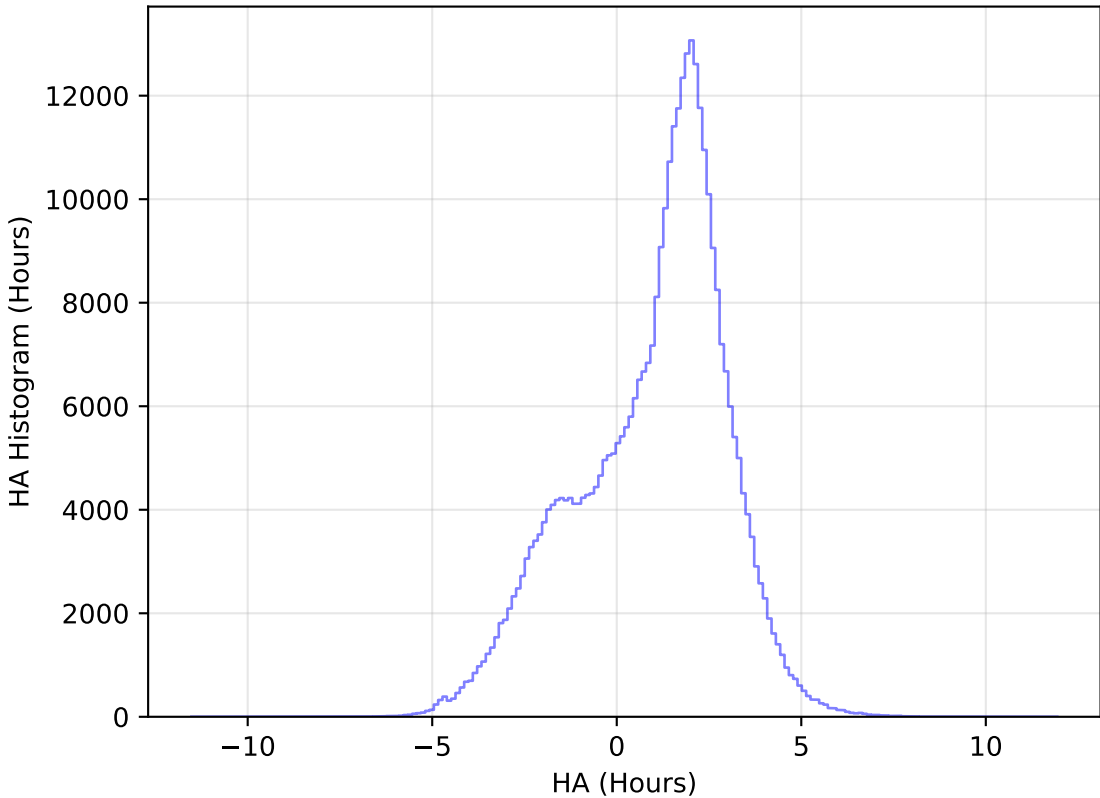
ddf_acor_sf20_lsf30_lsr50_v3.4_10yrs WFD y band: HA Histogram
