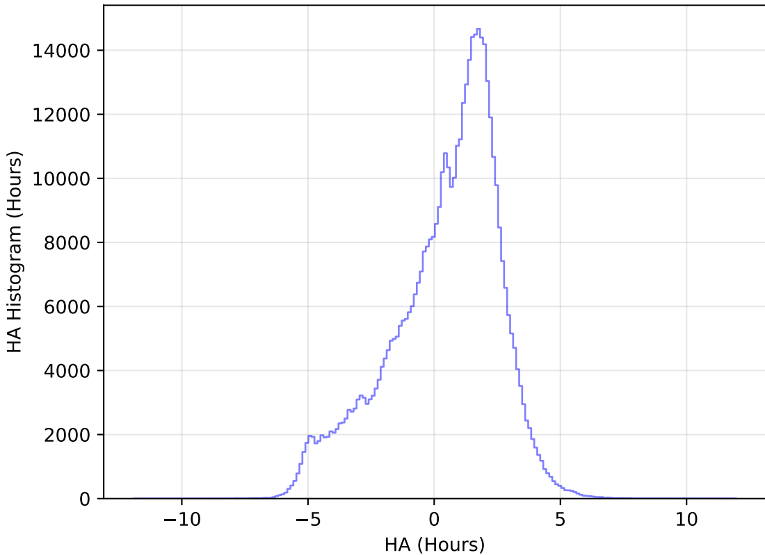
ddf_acor_sf20_lsf30_lsr50_v3.4_10yrs WFD r band: HA Histogram
