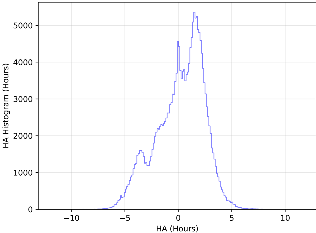
ddf_acor_sf20_lsf30_lsr50_v3.4_10yrs WFD g band: HA Histogram
