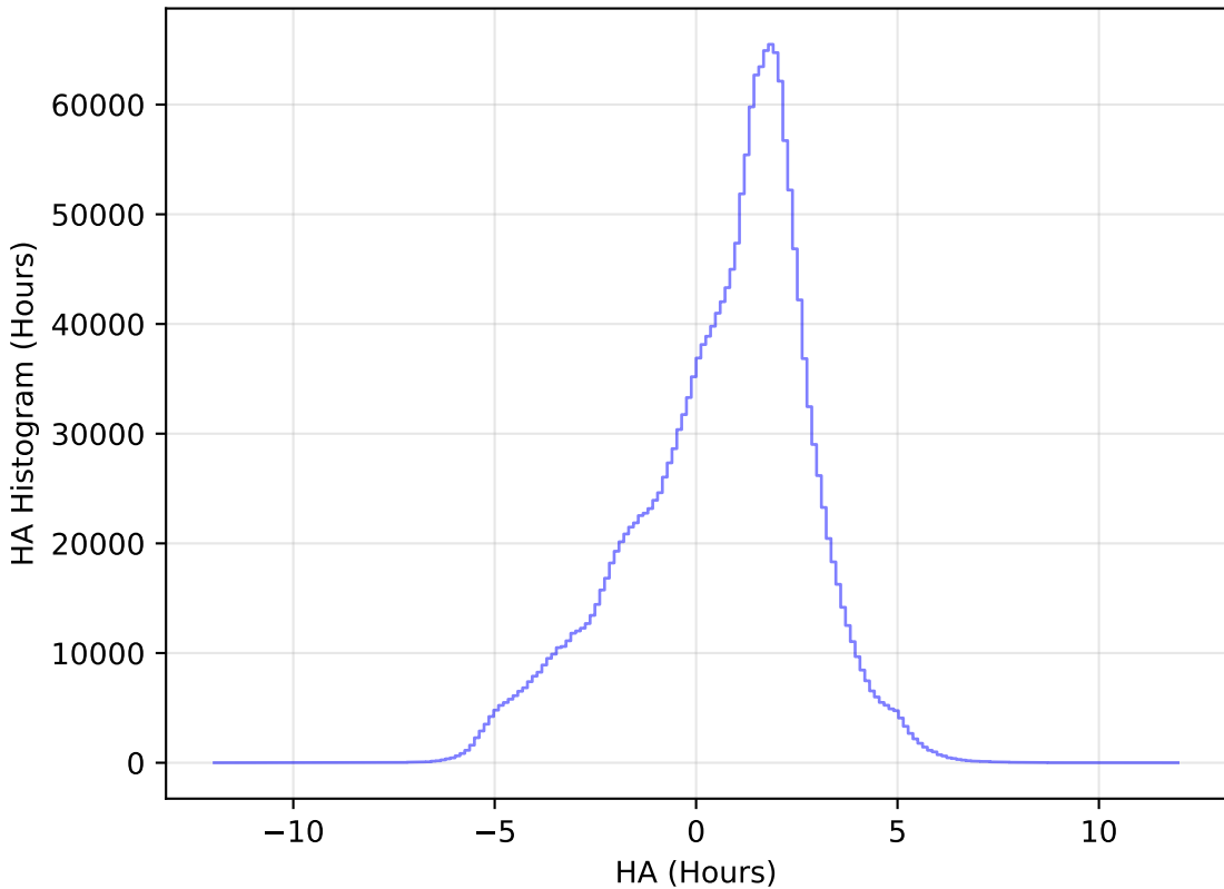
ddf_acor_sf20_lsf30_lsr50_v3.4_10yrs WFD all bands: HA Histogram
