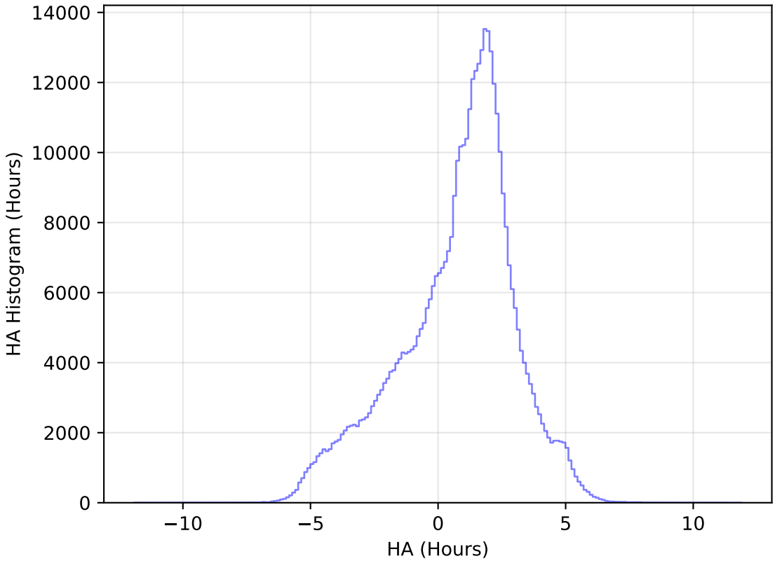
ddf_acor_sf20_lsf30_lsr50_v3.4_10yrs All sky z band: HA Histogram
