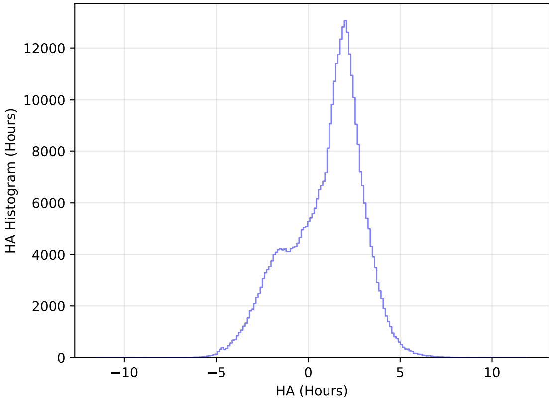
ddf_acor_sf20_lsf30_lsr50_v3.4_10yrs All sky y band: HA Histogram
