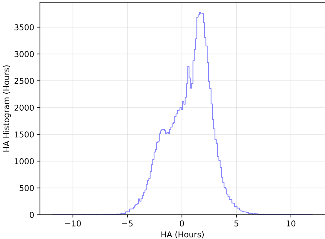
ddf_acor_sf20_lsf30_lsr50_v3.4_10yrs All sky u band: HA Histogram
