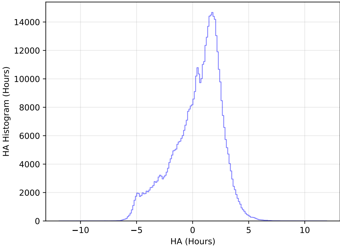
ddf_acor_sf20_lsf30_lsr50_v3.4_10yrs All sky r band: HA Histogram
