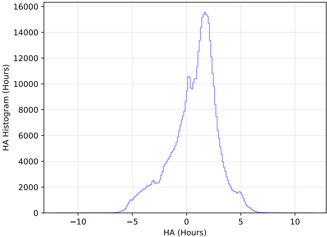
ddf_acor_sf20_lsf30_lsr50_v3.4_10yrs All sky i band: HA Histogram
