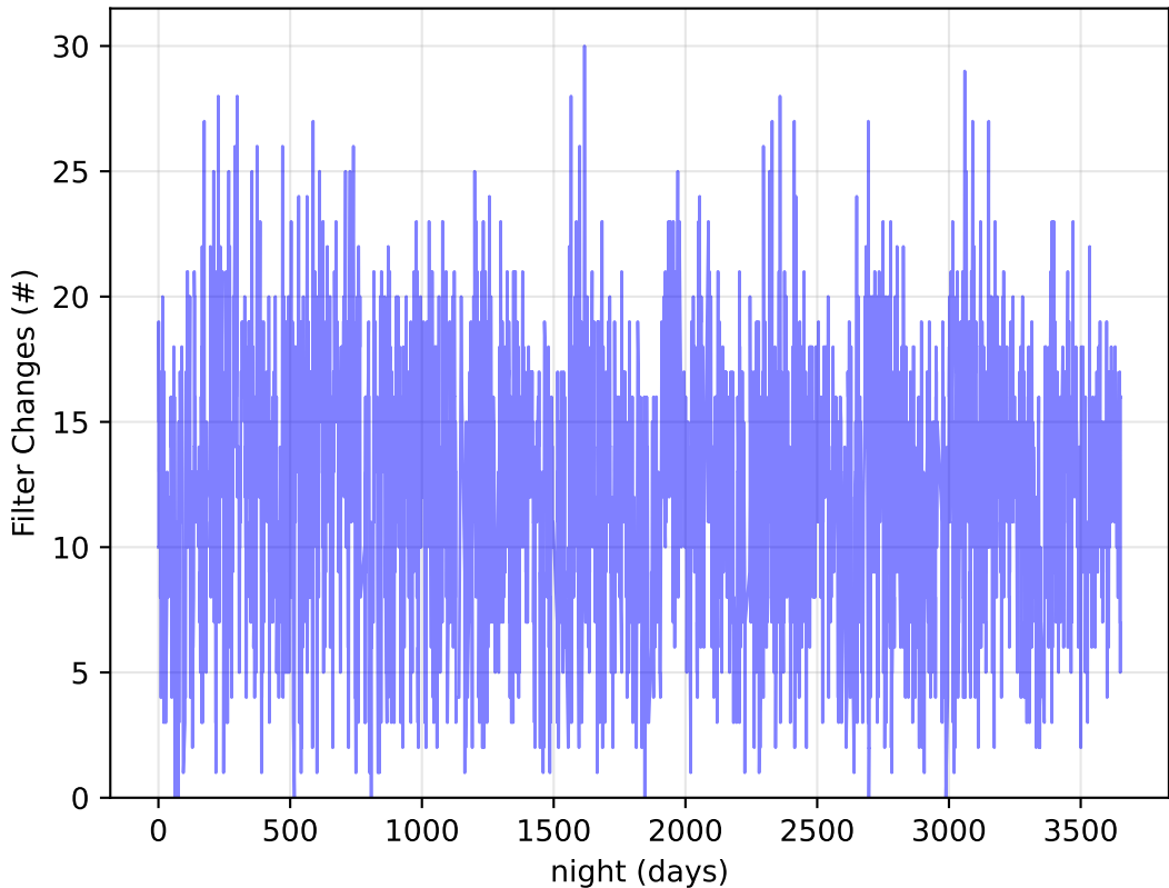
ddf_acor_sf20_lsf30_lsr50_v3.4_10yrs Per Night: Filter Changes
