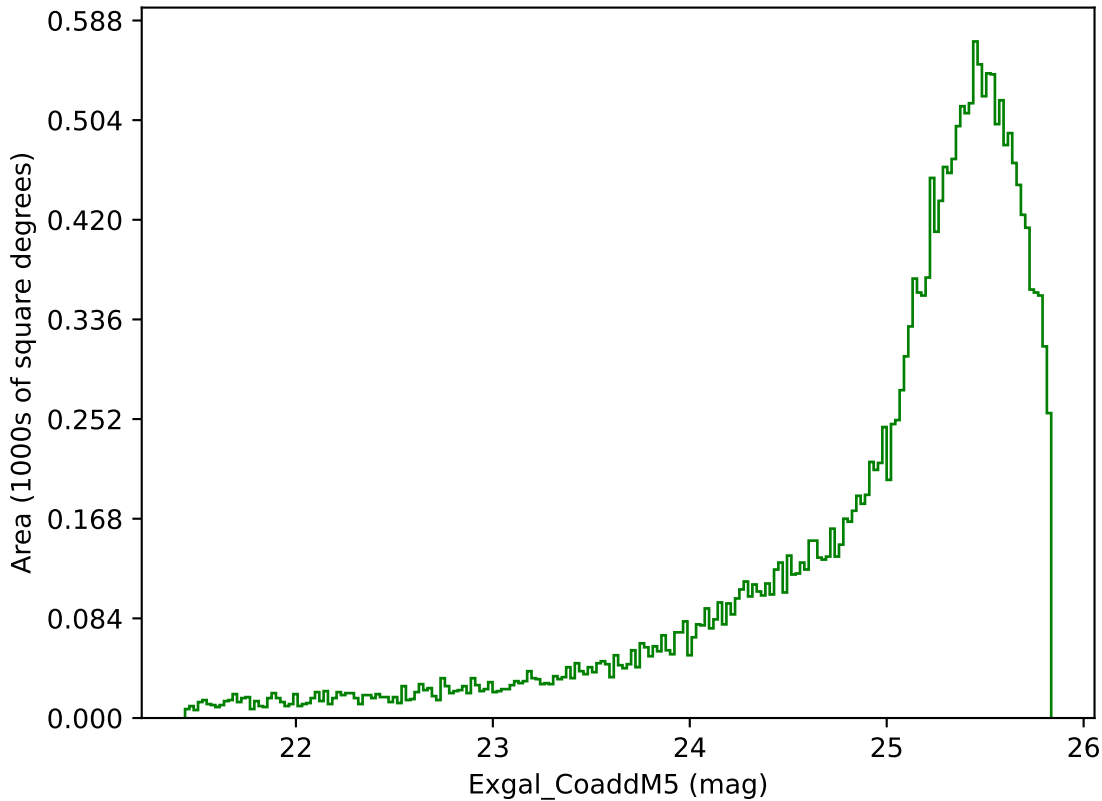
ddf_acor_sf20_lsf30_lsr50_v3.4_10yrs Yr 1 g band: Exgal_CoaddM5
