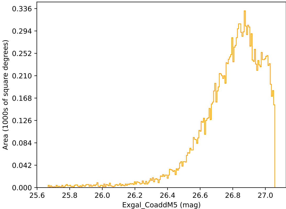
ddf_acor_sf20_lsf30_lsr50_v3.4_10yrs WFD r band: Exgal_CoaddM5
