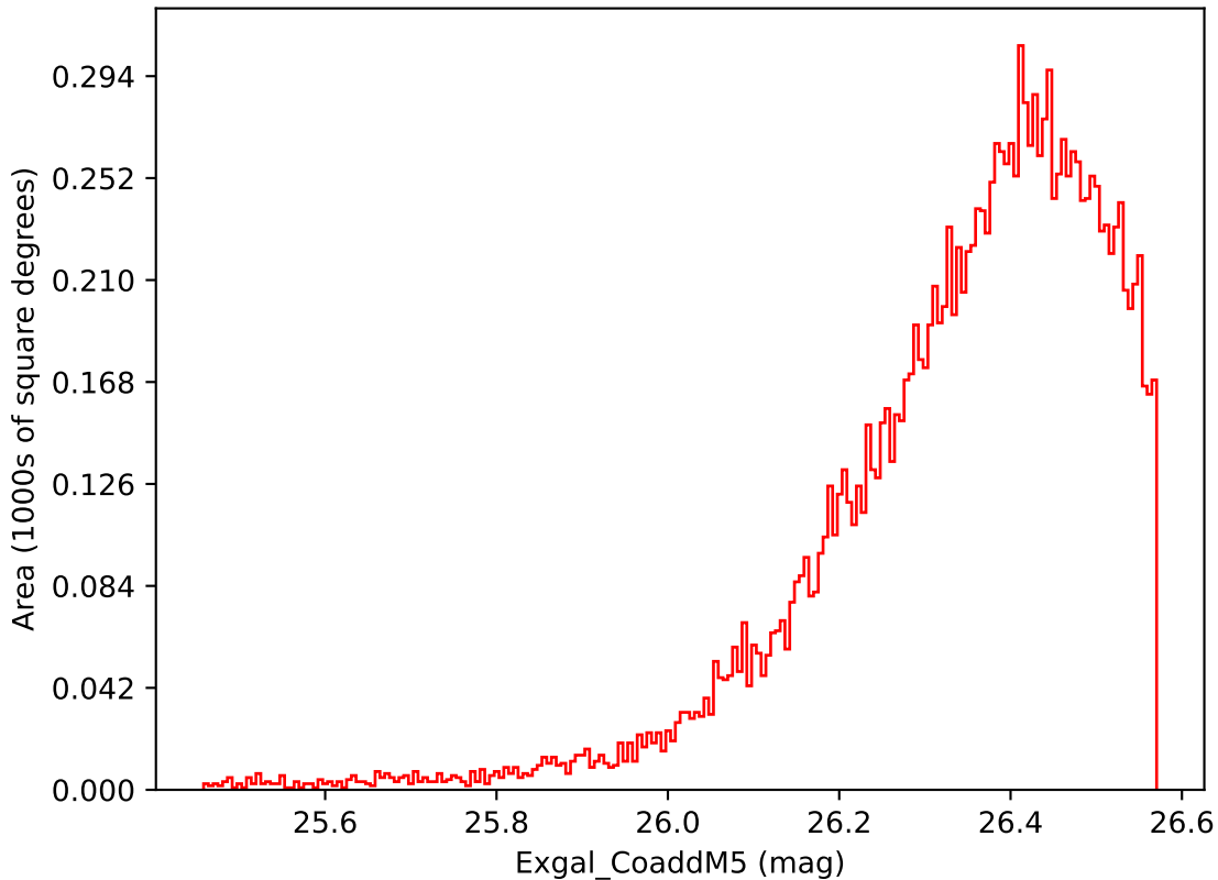
ddf_acor_sf20_lsf30_lsr50_v3.4_10yrs WFD i band: Exgal_CoaddM5
